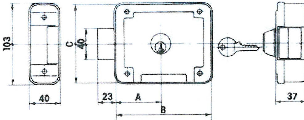
Horizontal mount
